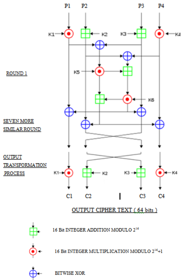
Figure1. Basic structure of IDEA Algorithm
