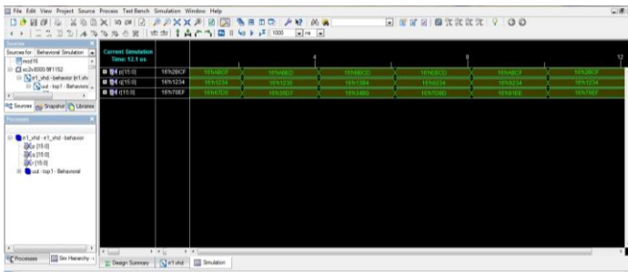
Figure 5. Simulation Waveform of Implemented Modulo Multiplier
