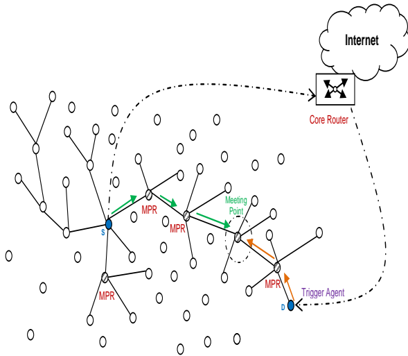
Fig.4. EEMDV protocol routing Architecture
