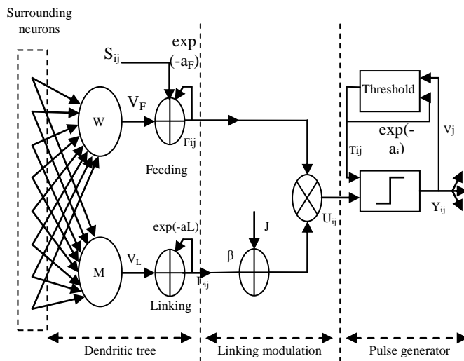
Fig. 1 Structure of PCNN
