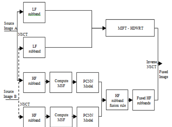
Fig. 2 Block diagram of MIFT – DWNRT Technique
