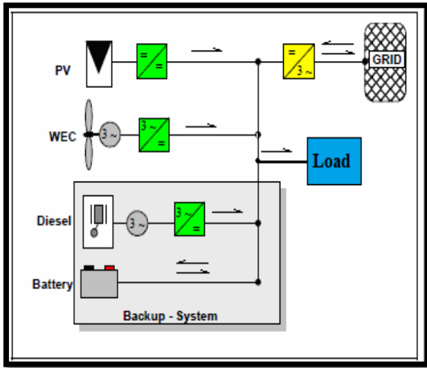
Figure 9 Centralized DC-bus architecture
