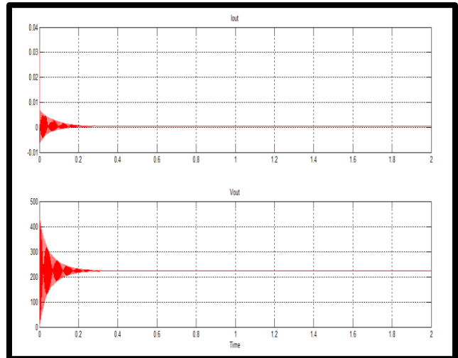
Figure 147 Stable output for Solar with MPPT
