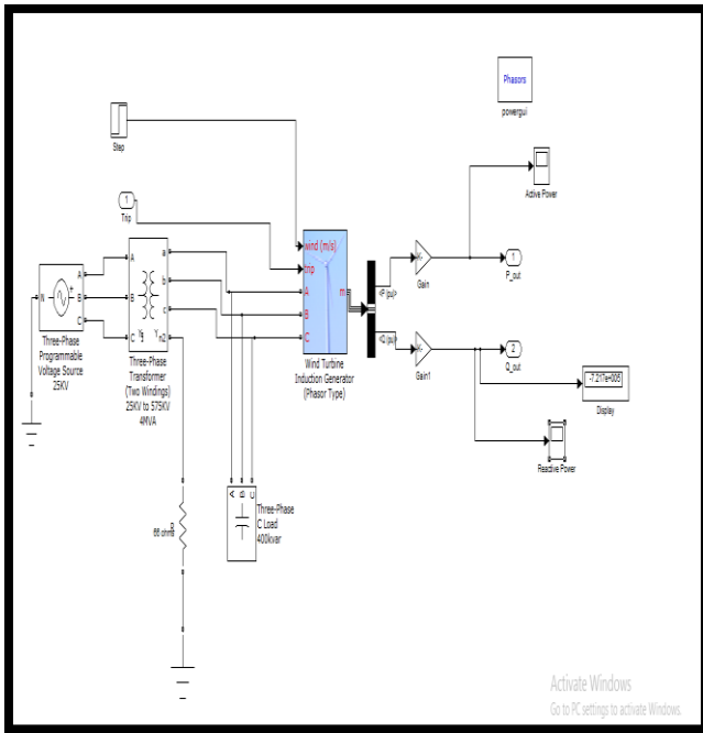
Figure 19 Wind Power Plant Simulation
