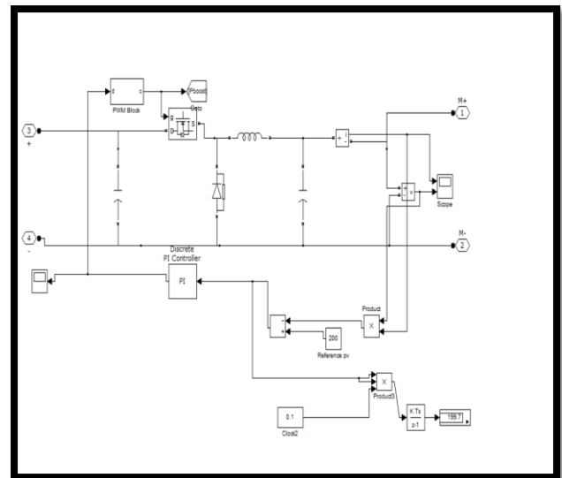
Figure 92 Solar MPPT and Boost converter System
