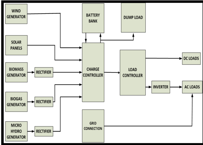
Figure 6 Basic Diagram of Hybrid System
