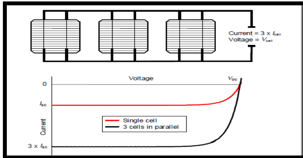
Figure 3 Parallel connection of cells, with resulting current-voltage characteristic
