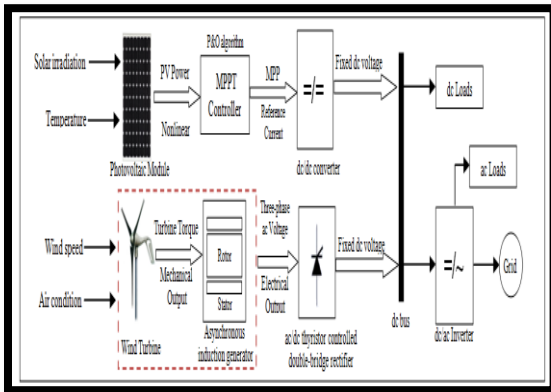
Figure 10 Block diagram of the proposed system
