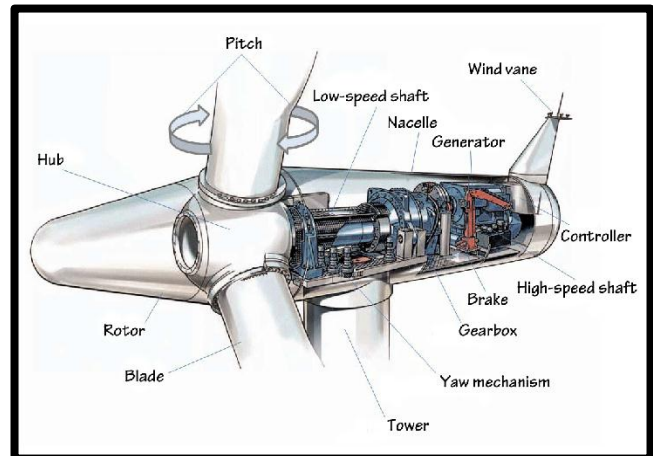
Figure 4 Major Component of Wind Turbine
