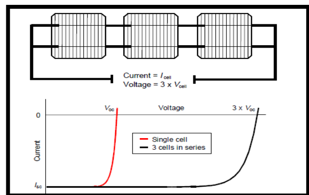
Figure 2 Series connection of cells, with resulting current-voltage characteristic
