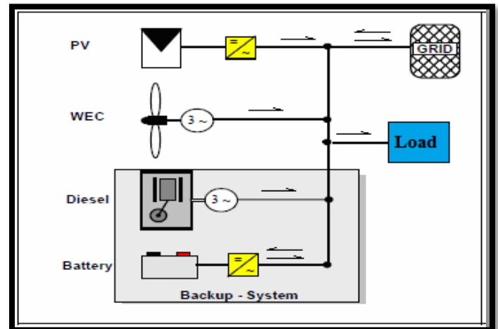
Figure 8 Centralized AC-bus architecture
