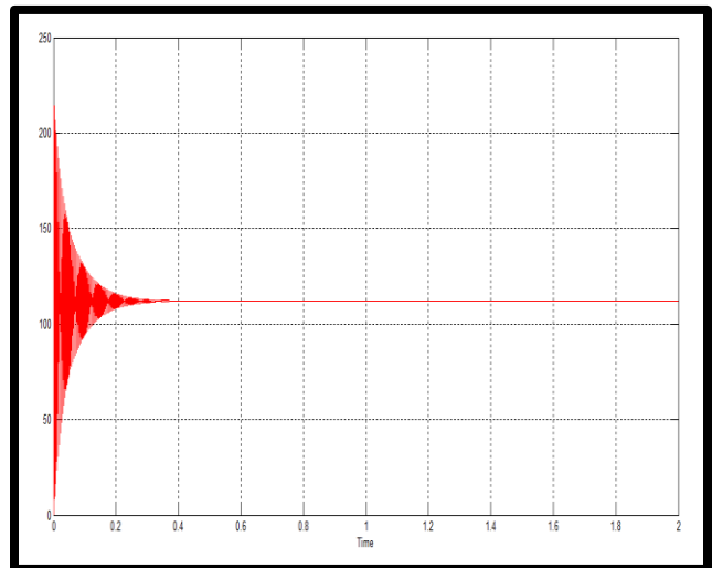
Figure 136 Solar D.C stable Output
