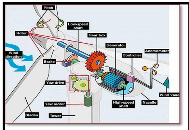
Figure 5 The Main component of a Wind Turbine can be classified as i) Tower ii) Rotor System iii) Generator iv) Yaw v) Control System vi) Breaking and Transmission System
