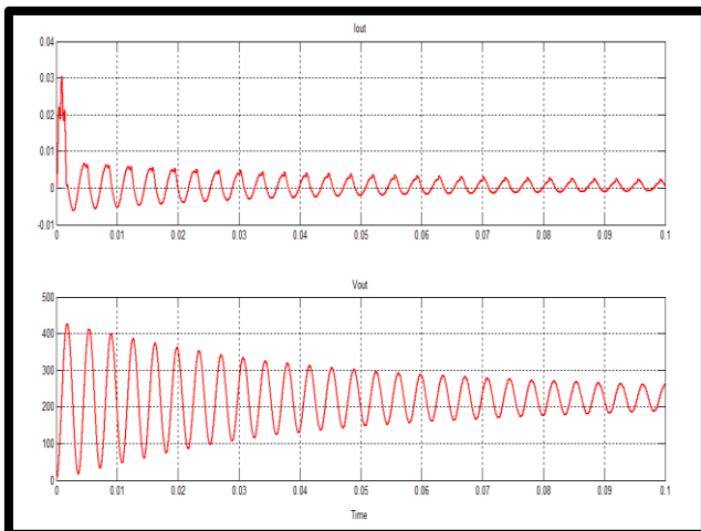
Figure 125 Solar Unstable Output
