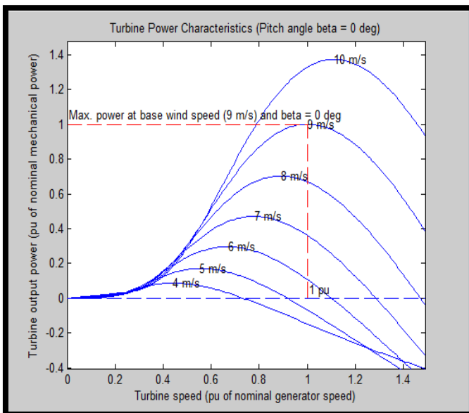
Figure 160 Mechanical Power and Turbine Speed
