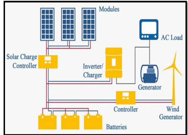
Figure 7-b Solar-Wind Hybrid System
