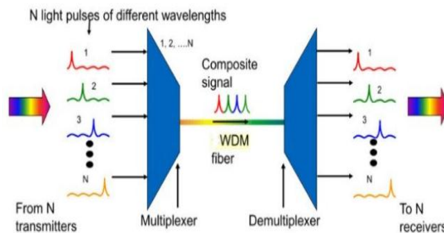
Fig1: WDM Network Architecture
