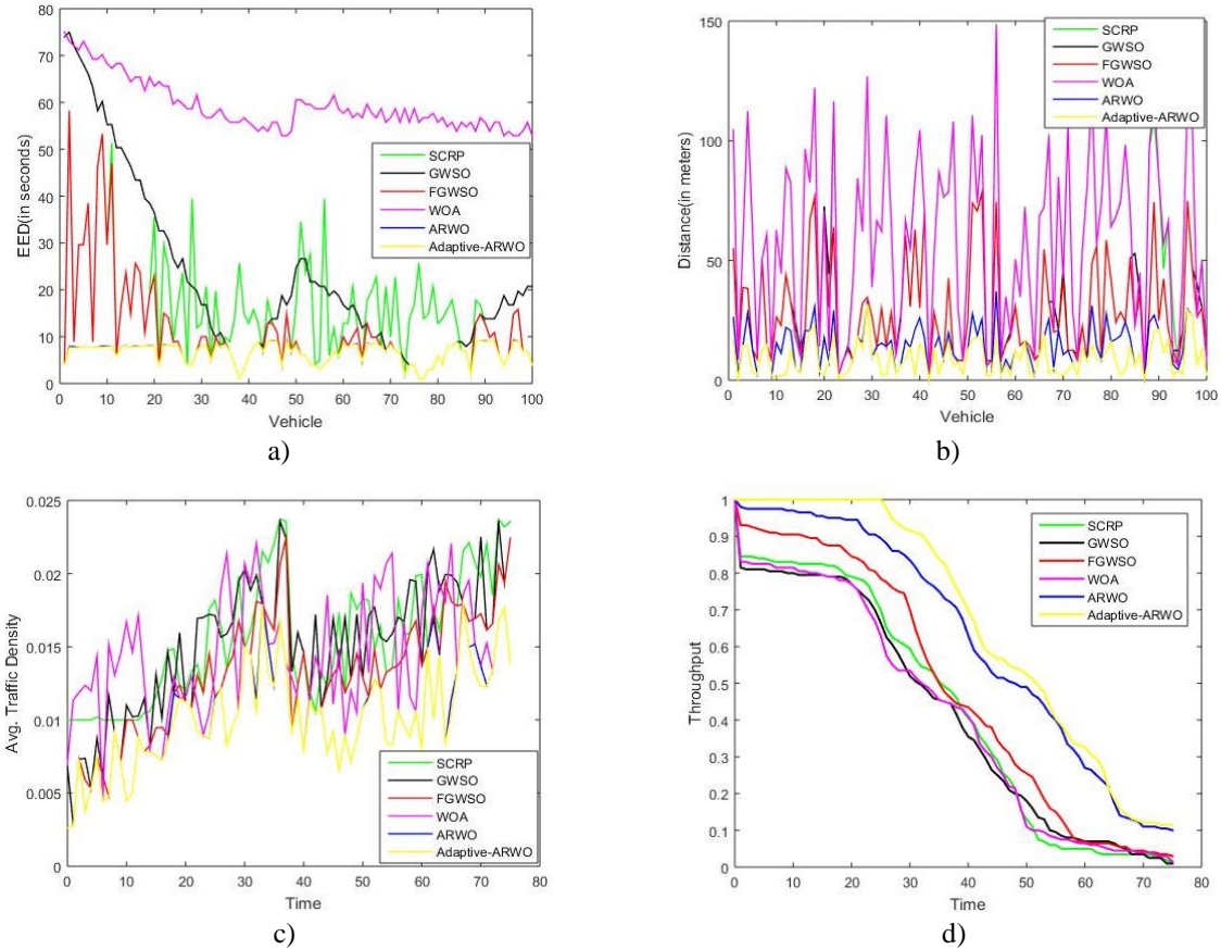
Figure 3. Analysis using setup2 a) EED b) Distance c) Average Traffic density d) Throughput
