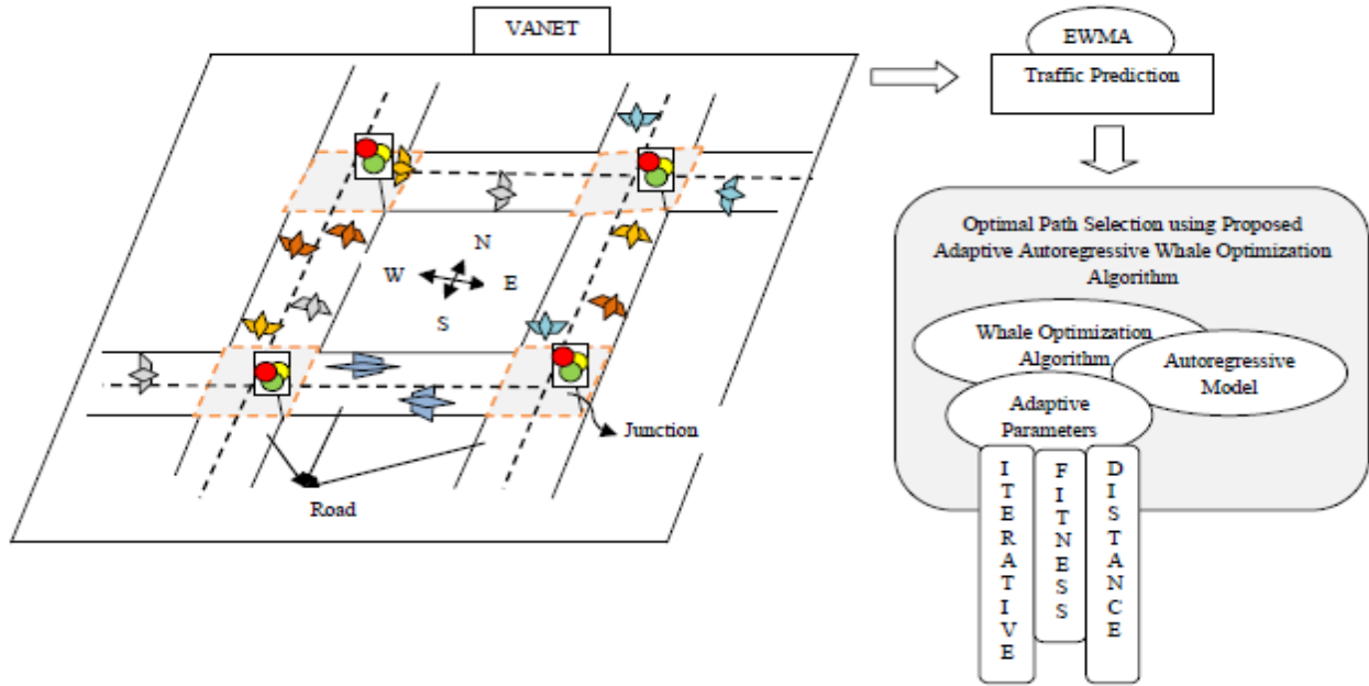
Figure 1. Traffic-aware routing using the proposed algorithm
