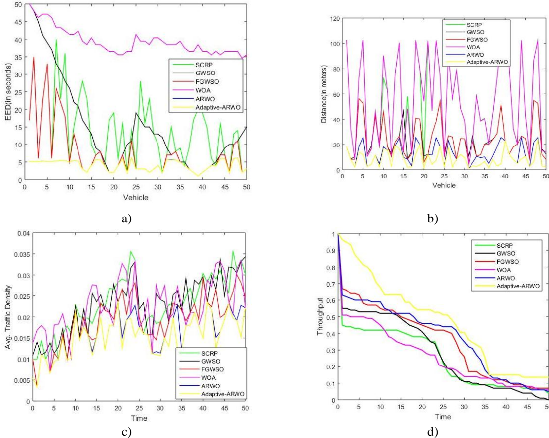
Figure 2. Analysis using setup1 a) EED b) Distance c) Average Traffic density d) Throughput
