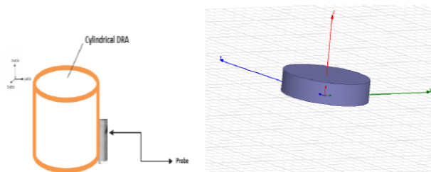
CYLINDRICAL DIELECTRIC RESONATOR ANTENNA (DRA) FOR GPS
