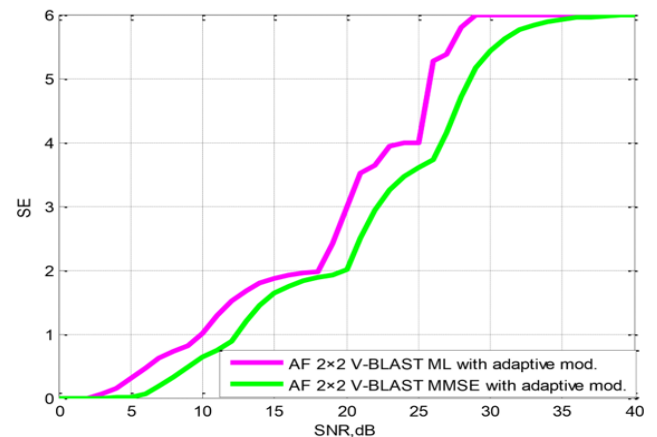
Fig. 14. Throughput performance of adaptive modulation cooperative 2x2 V-BLAST MIMO using MMSE and ML detection.
