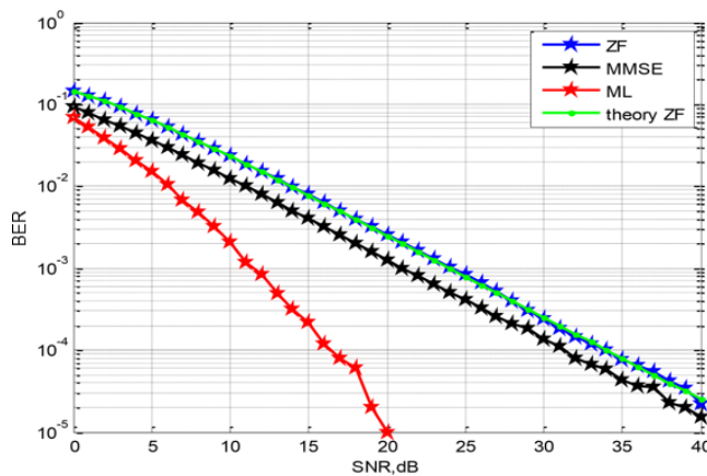
Fig. 3. BER performance of 2x2 V-BLAST MIMO using BPSK modulation for different detection scheme
