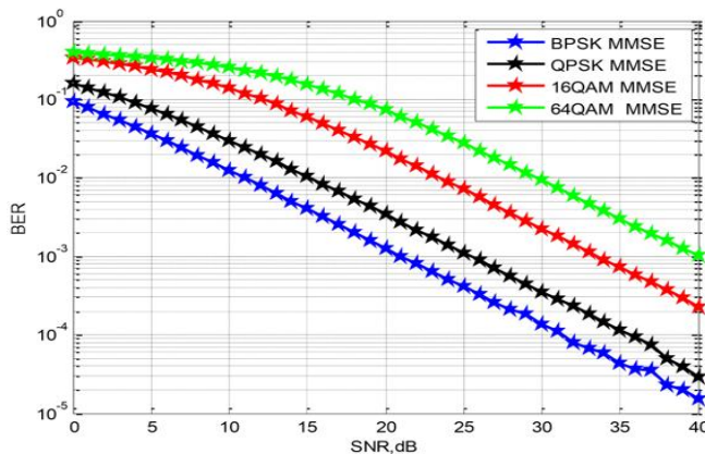
Fig. 4. BER performance of 2x2 V-BLAST MIMO system using MMSE detection for different modulation
