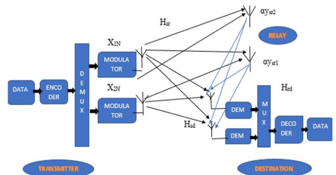
Fig. 2. System Model of Cooperative MIMO
