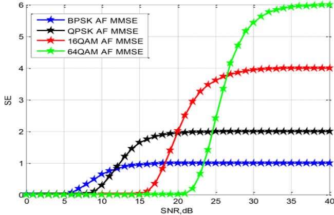
Fig. 11. Throughput performance Cooperative 2x2 V-BLAST system using MMSE detection for different modulation
