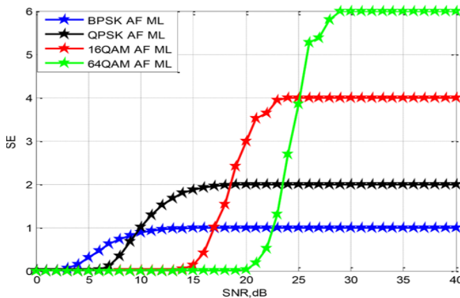
Fig. 8. Spectral efficiency of adaptive modulation 2x2 V-BLAST MIMO using ML detection
