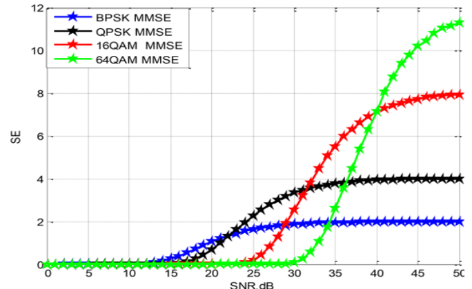
Fig. 5. Spectral efficiency of 2x2 V-BLAST MIMO using MMSE detection for different modulation.
