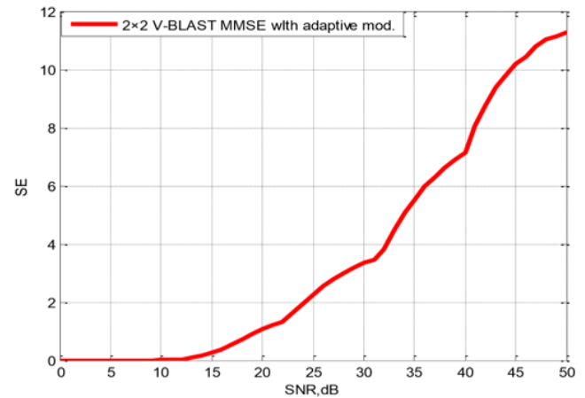
Fig. 6. Spectral efficiency of adaptive modulation 2x2 V-BLAST MIMO using MMSE detection
