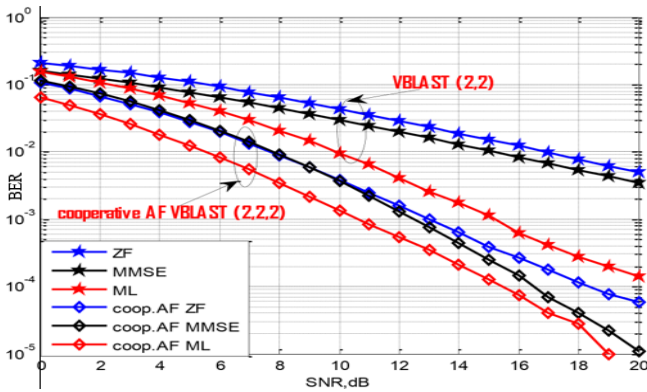
Fig. 15. BER Performance curves of cooperative 2x2 V-BLAST MIMO system for different detectors (ML, ZF and MMSE).
