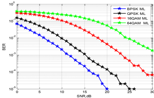
Fig. 7. BER performance of 2x2 V-BLAST MIMO system using ML detection for different modulation
