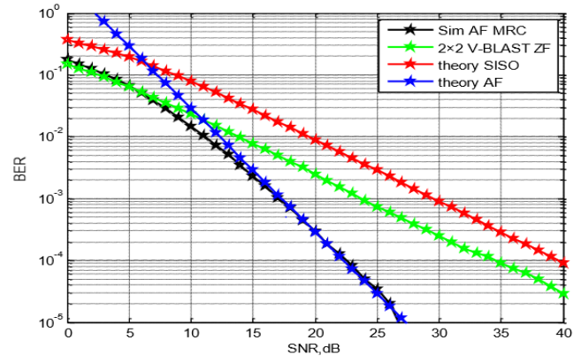
Fig. 9. BER performance of cooperative diversity, 2x2 V-BLAST MIMO, and SISO with BPSK modulation.
