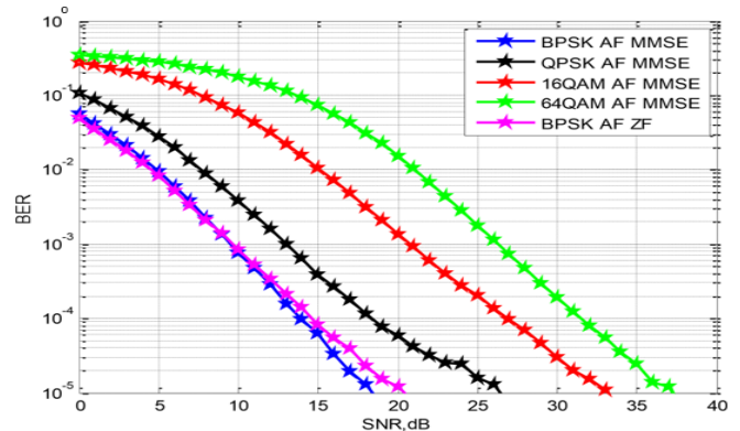
Fig. 10. BER Performance of Cooperative 2x2 V-BLAST MIMO system using MMSE and ZF detections for different modulation schemes
