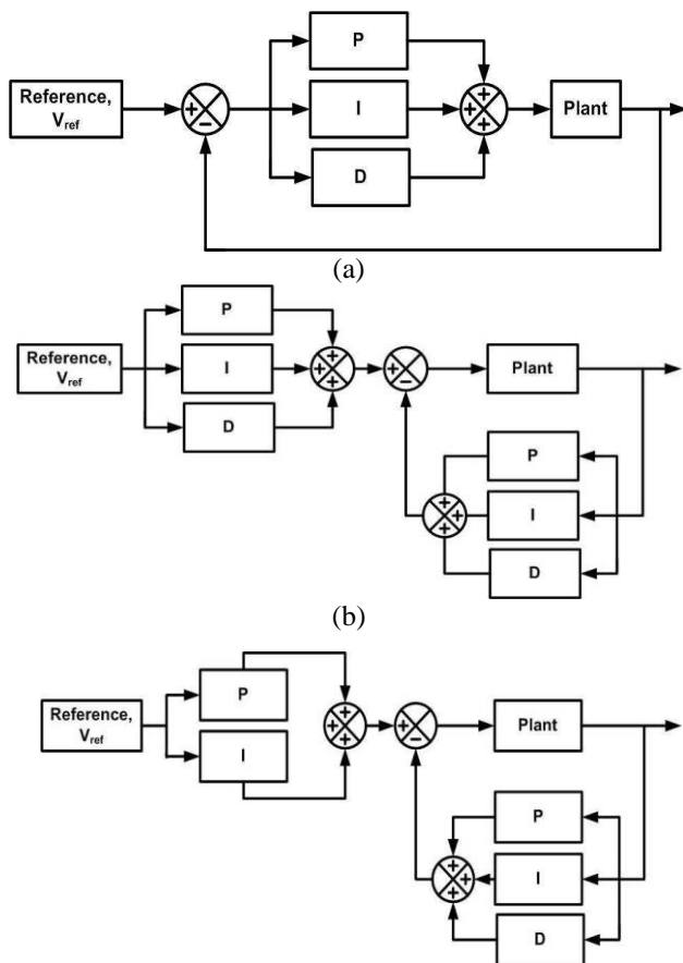
Fig. 4. Typical PID control Structure
