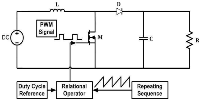
Fig. 2. Conventional Boost Converter
