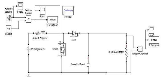
Fig. 7. MATLAB-Simulink model of conventional Boost converter
