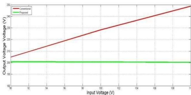
Fig. 9. Output voltage comparison between conventional and proposed Boost converter
