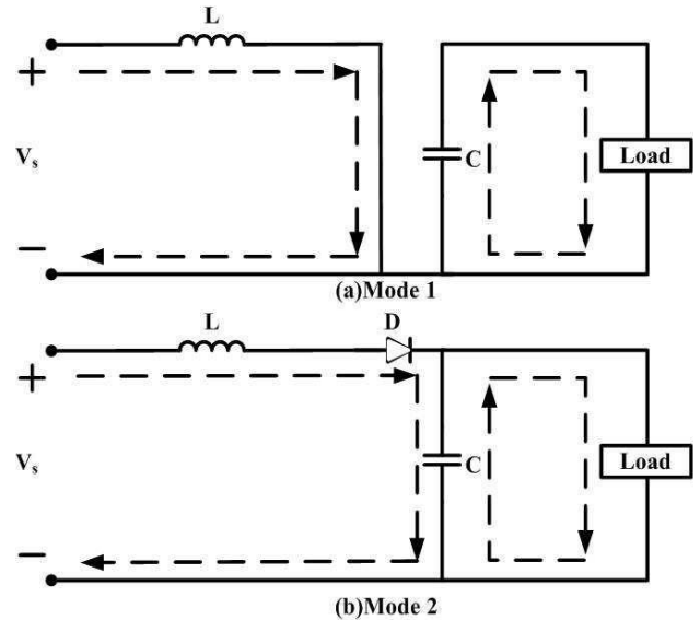
Fig. 3. Mode of operation of Boost Converter
