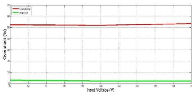
Fig. 10. Percentage overshoot comparison between conventional and proposed Boost converter
