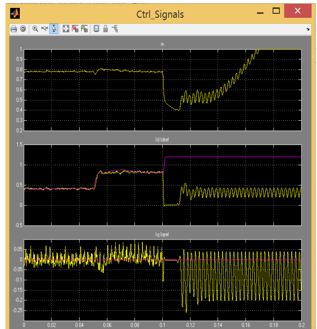
Figure 4: Output waveform of the AC/DC Three Level Control Signal PWM Converter
