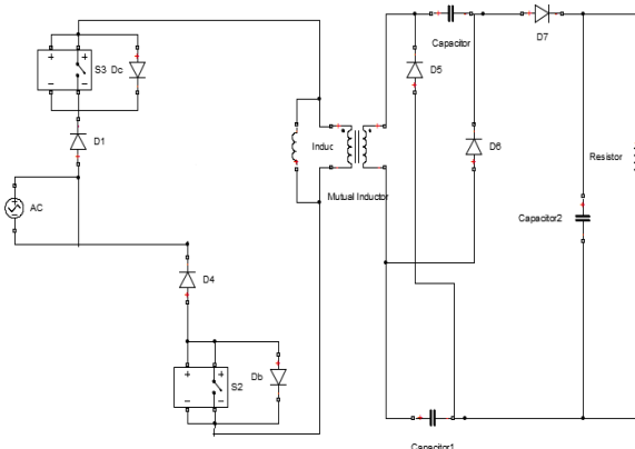
Figure 9: Circuit operation in mode-II
