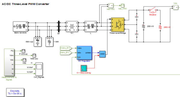
Figure 2: MATLAB Simulink Model of AC/DC Three Level PWM Converter
