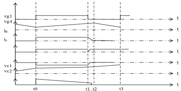
Figure 7: Waveforms of AC-DC Converter using Switching Technique
