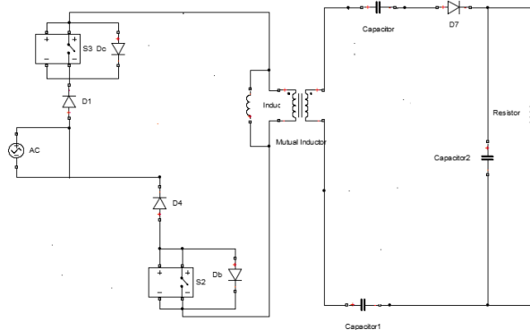
Figure 8: Circuit operation in mode-I
