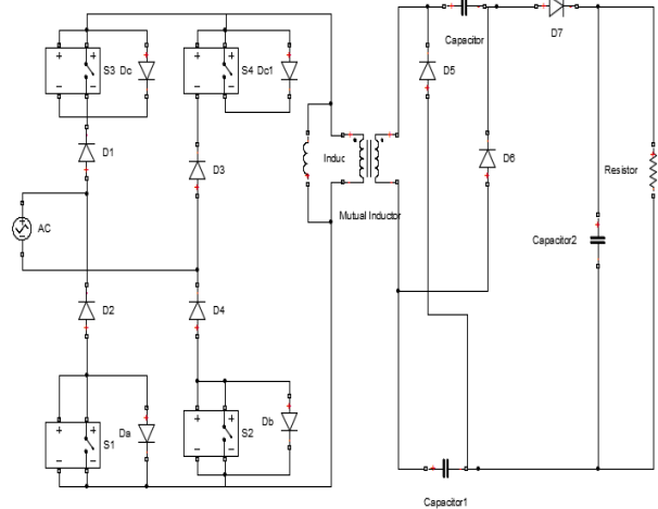
Figure 6: Circuit of Proposed Converter using Switching Capacitor Technique
