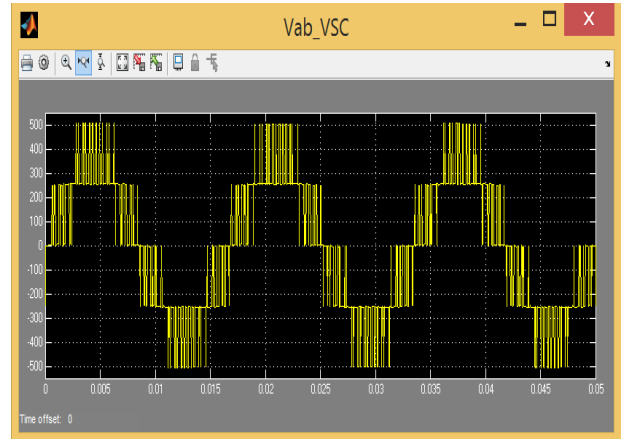
Figure 3: Output waveform of the AC/DC Three Level PWM Converter
