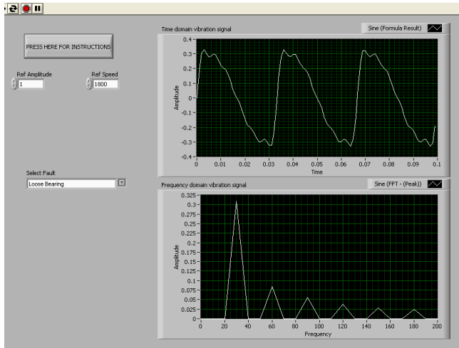
Fig.7 Loose Bearing
