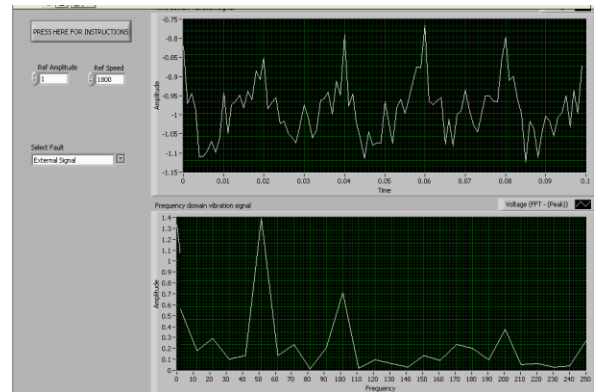
Fig. 14 SCIM Vibrations at MI=1 and f=50Hz
