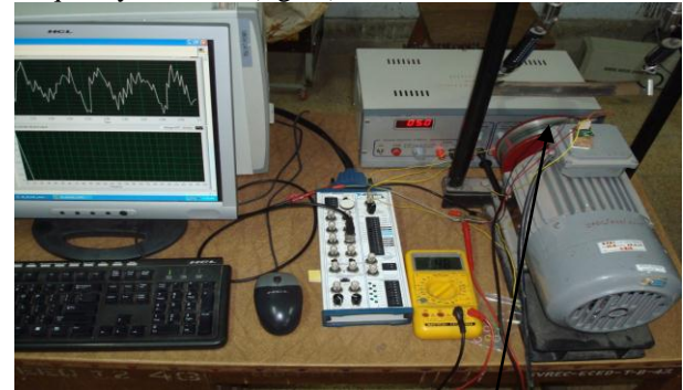
ADXL 203 Fig. 13 Arrangement on SCIM
