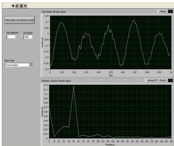
Fig. 11 Least vibration level (Magnet attached at free end)
