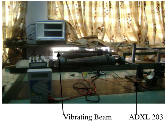
Fig. 10 Arrangement on Vibrating Beam
