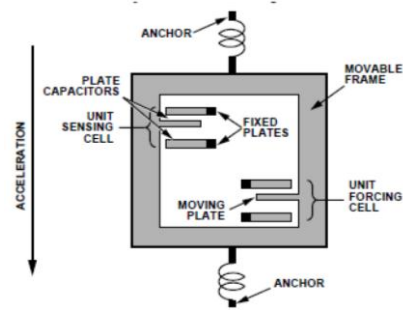
Fig. 9 Internal Arrangement in IC Accelerometer
