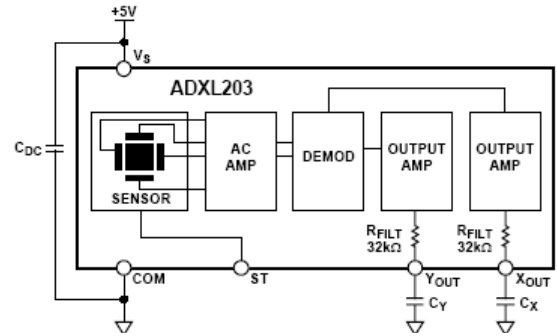
Fig. 8 Block diagram of ADXL 203[5]
