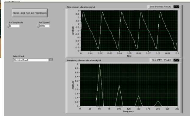
Fig.5 Electrical Fault
