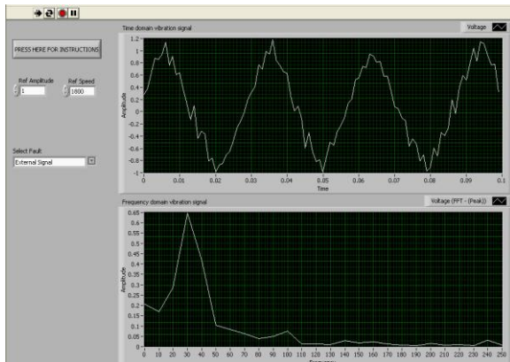
Fig. 12 Highest vibration Level (Magnet attached at hinge)
