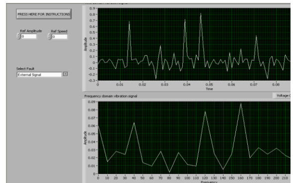
Fig. 15 SCIM Vibrations at MI=1 and f=40Hz
