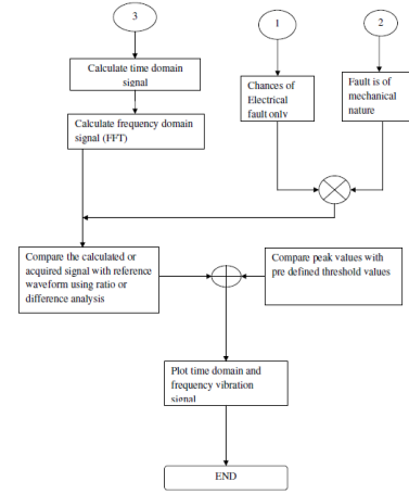
Fig.4 Flow chart for User Interface and fault calculation
