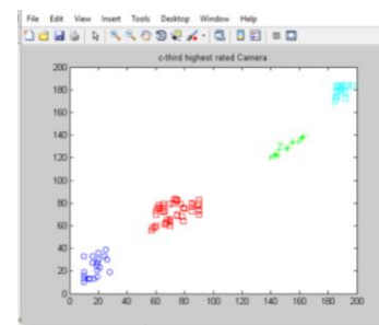
Fig 4.1 Clustering result
