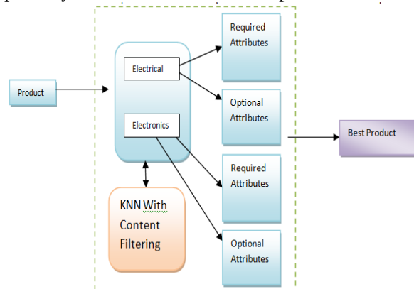
Fig 1.1 Proposed model for product promotion
