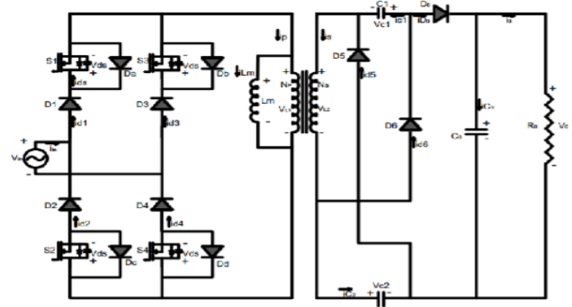
Figure 6: Circuit of Proposed Converter using Switching Capacitor Technique
