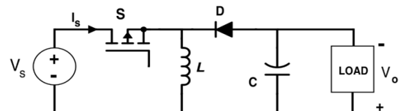
Figure 4: Block Diagram of Buck-Boost Converter
