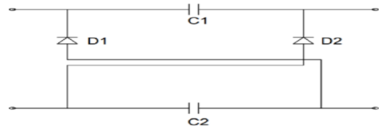
Figure 7: Switched Capacitor Technique
