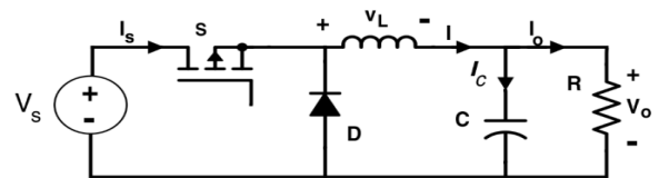
Figure 3: Block Diagram of Buck Converter
