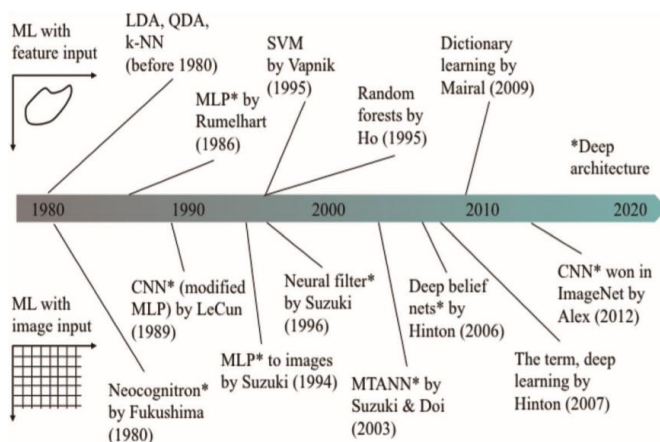
Fig. 5 The history of ML in the fields of computer vision and medical imaging. There are two distinct ML approaches in these fields. Before the popularity of “deep learning” starting in 2013, ML with feature input (feature-based ML) was dominant in the fields. After that, ML with image input (image-based ML) including deep learning gained enthusiastic popularity, but it has a long history
