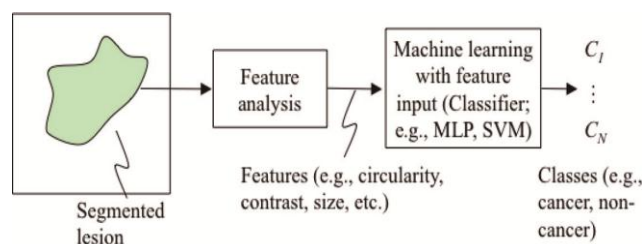
Fig. 1 Standard ML for classifying lesions (i.e., ML with feature input or feature-based ML) in the field of computer vision before the introduction of deep learning. Features (e.g., circularity, contrast, and effective diameter) are extracted from a segmented lesion in an image. Those features are
