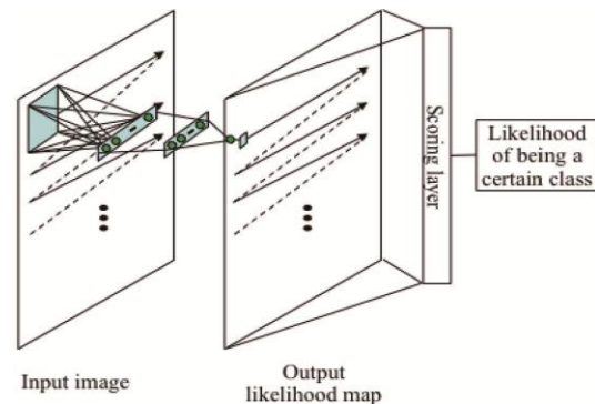
Fig. 6 Architecture of an MTANN consisting of an ML model (e.g., linear-output-layer ANN regression) with sub region (or image patch, local kernel) input and single-pixel output. The entire output image representing a likelihood map is obtained by scanning with the input sub region of the MTANN in a convolutional manner on the entire input image. A scoring layer is placed in the end to convert the output likelihood map into a single score that represents the likelihood of being a certain class for a given input image.
