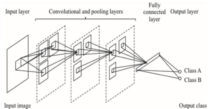
Fig. 2 Architecture of a CNN. The layers in the CNN are connected with local shift-invariant inter-connections (or convolution with a local kernel). The input and output of the CNN are images and class labels (e.g., Class A and Class B), respectively.
