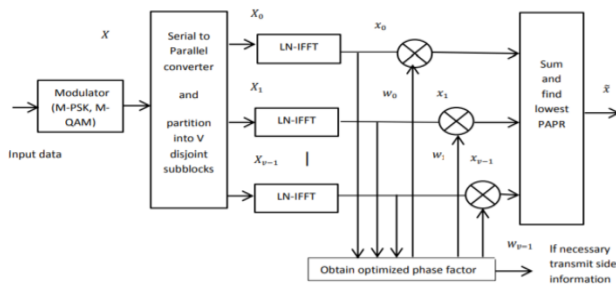
Figure 2: Block diagram of the PTS scheme with two transmit antennas
