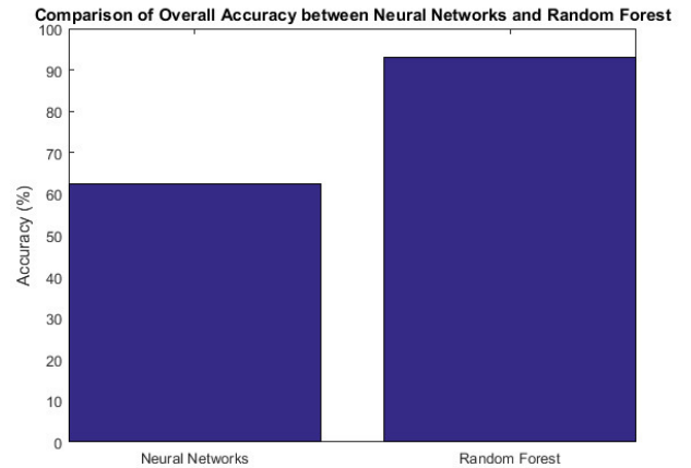
Fig 2: Comparison between accuracies of Random forest and scaled conjugate gradient
