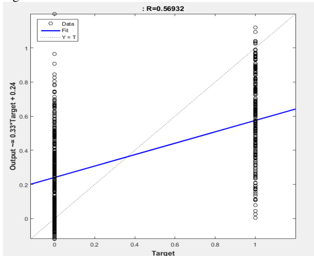
Fig 1: Regression plot for the scaled conjugate gradient
