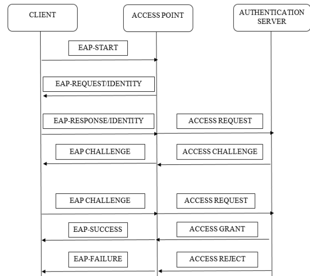
Figure 3. EAP Flow Diagram
