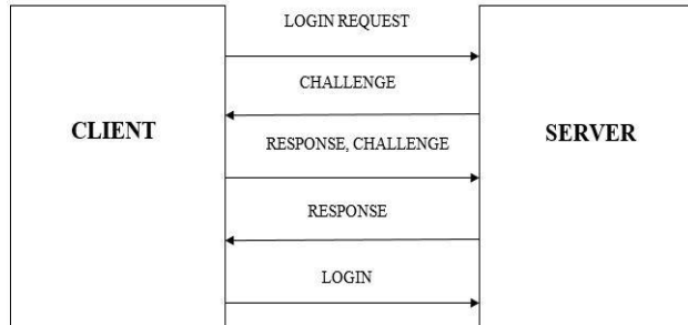
Figure 4. PAP Flow Diagram
