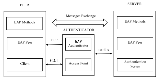
Figure 2. EAP Protocol Stack
