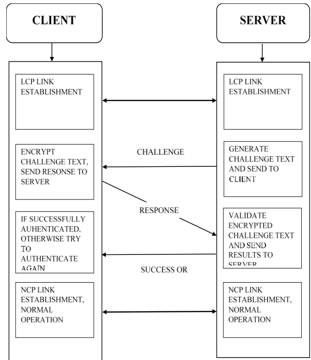
Figure 5. CHAP 3-way Handshake
