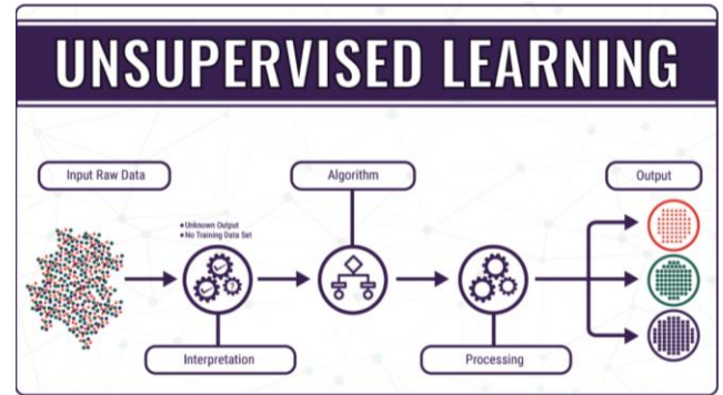
Fig. 2 Unsupervised Learning
