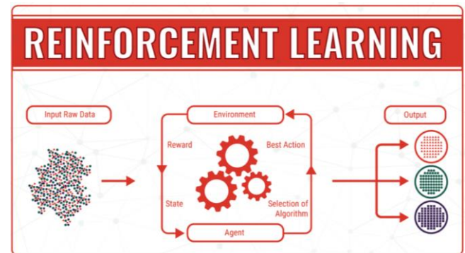
Fig. 3 Reinforcement Learning
