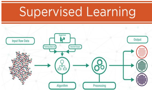
Fig.1 Supervised Learning
