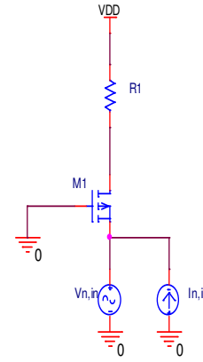
Fig. 10. Input noise sources for the common gate stage.
