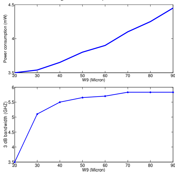
Fig. 7. The power consumption (top) and the bandwidth (bottom) as a function of channel width of M_9 ( W_9 ).
