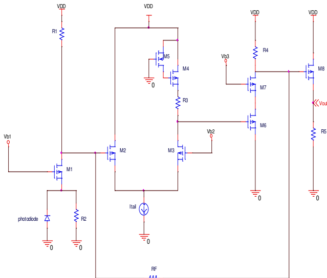
Fig. 2. Topology of proposed TIA.
