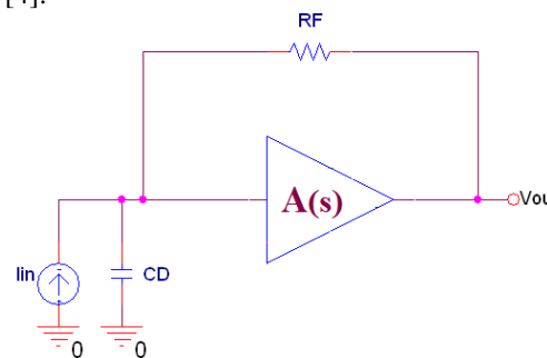
Fig. 1. Topology of a shunt-feedback TIA
