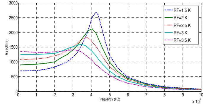
Fig. 5. The trans-resistance of proposed TIA as a function of frequency for different values of R_f .
