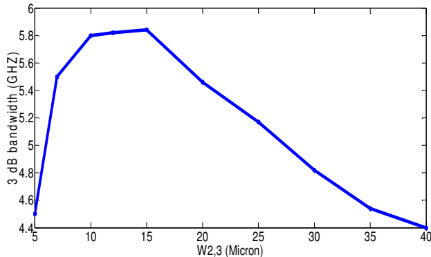
Fig. 6. The bandwidth of proposed TIA as a function of channel width of M_{2,3} ( W_{2,3} ).
